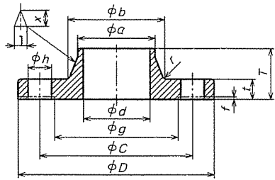
WN of nominal size 10A to 1500A
