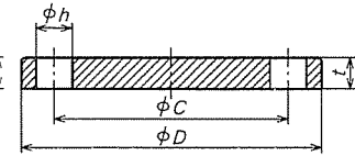
BL of nominal size 10A to 1500A
